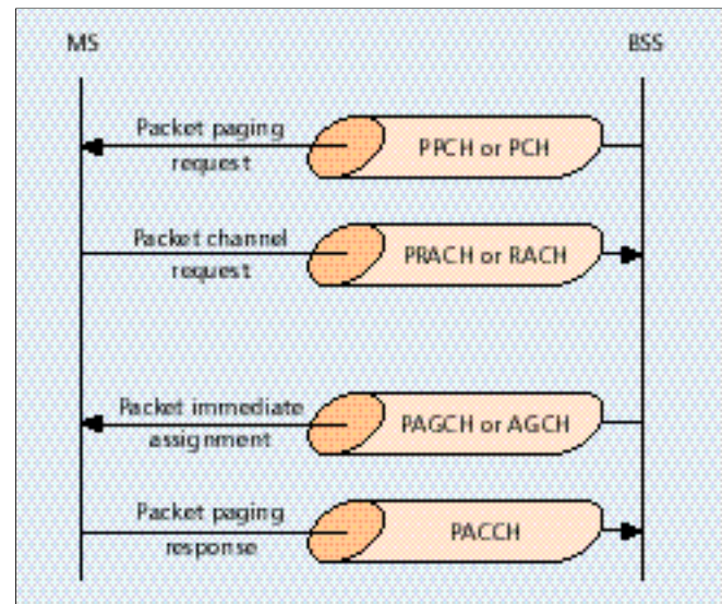
■ FIGURE 9. Paging (mobile terminated packet transfer).
