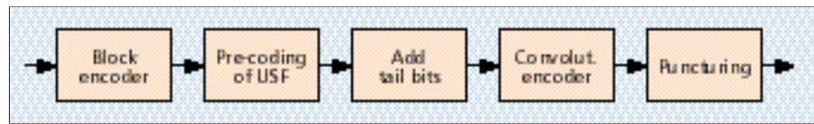
■ FIGURE 11. Encoding of GPRS data packets.
