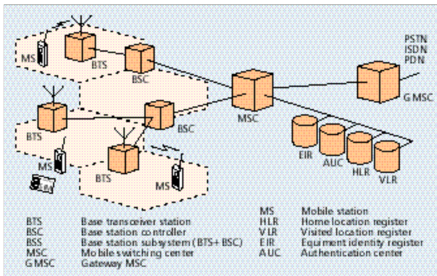
■ FIGURE 1. GSM system architecture with essential components.
