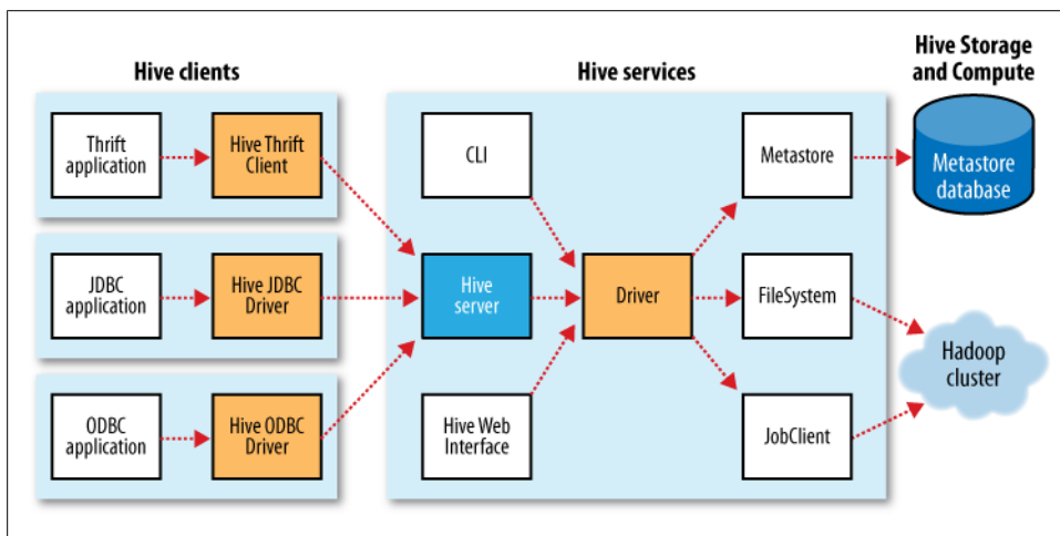
Figure 12-1. Hive architecture
